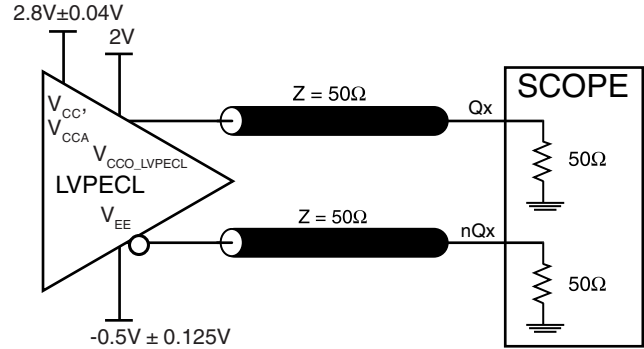
3.3V CORE/2.5V LVPEACL OUTPUT LOAD AC TEST CIRCUIT
