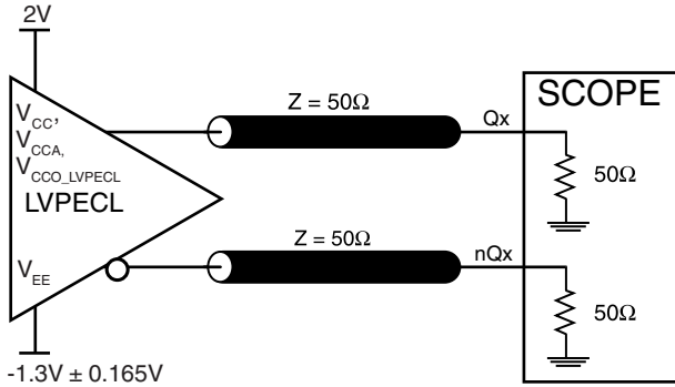
3.3V CORE/3.3V LVPEACL OUTPUT LOAD AC TEST CIRCUIT
