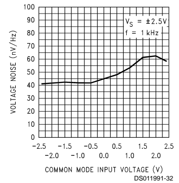
Input Voltage Noise vs Input Voltage (5V)
