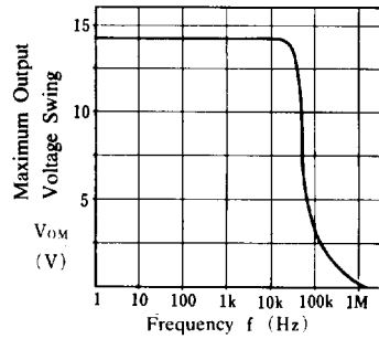
Maximum Output Voltage Swing vs. Frequency
