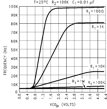
VHC4046 V_{CO,in} vs f_{OUT} V_{CC} = 4.5V
