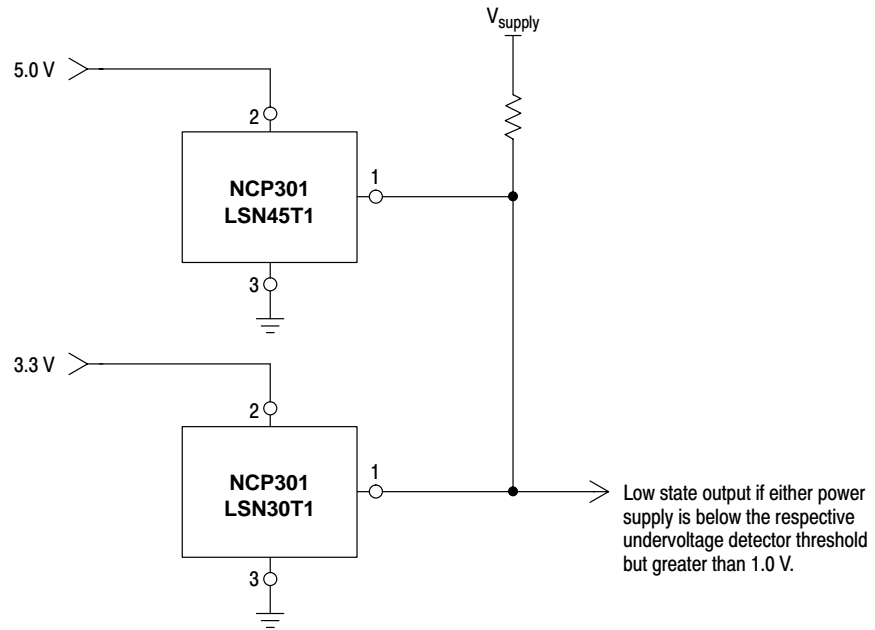
Figure 24. Dual Power Supply Undervoltage Supervision
