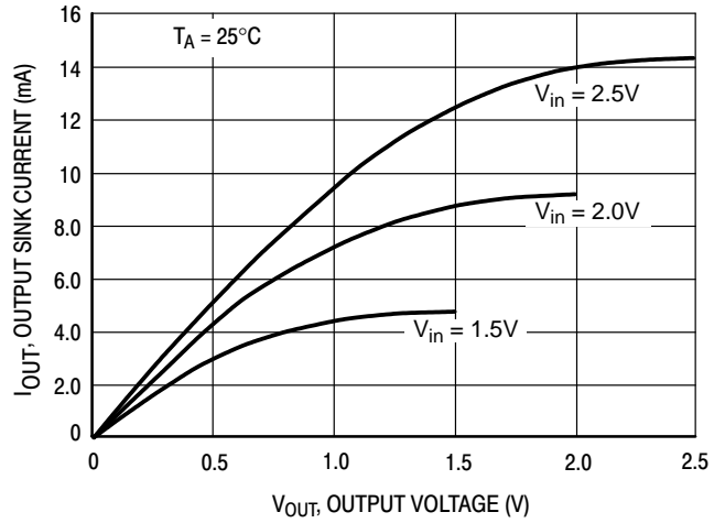
Figure 9. NCP300L/1L Series 2.7 V Reset Output Sink Current versus Output Voltage
