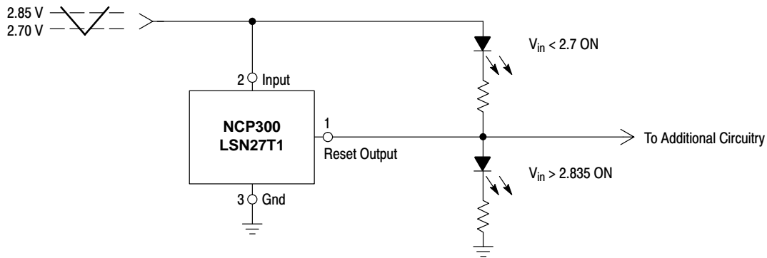
Figure 22. Battery Charge Indicator (NCP300 Series)
