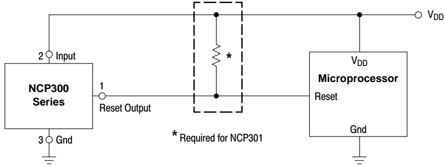
Figure 21. Microprocessor Reset Circuit (NCP300 and NCP301 Series)
