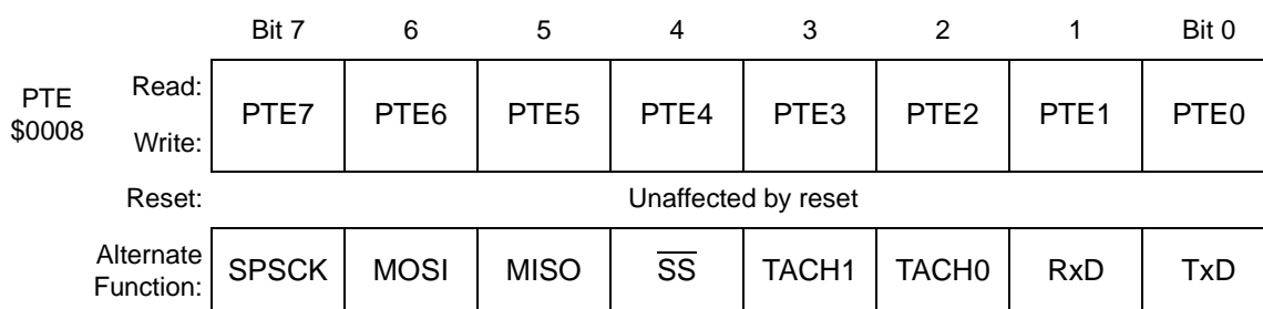
Figure 19-13. Port E Data Register (PTE)
