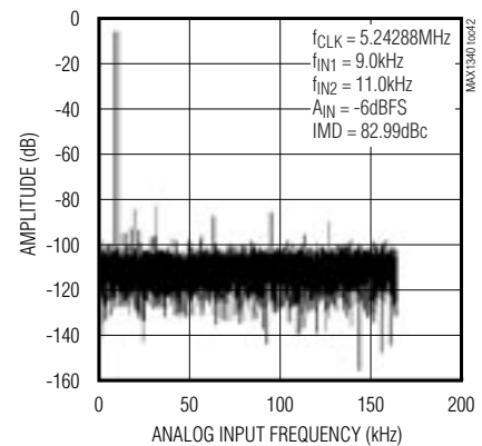
ADC IMD PLOT
