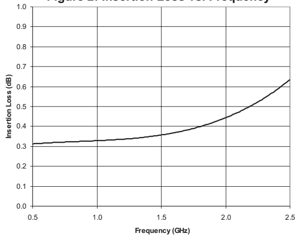
Figure 2: Insertion Loss vs. Frequency
