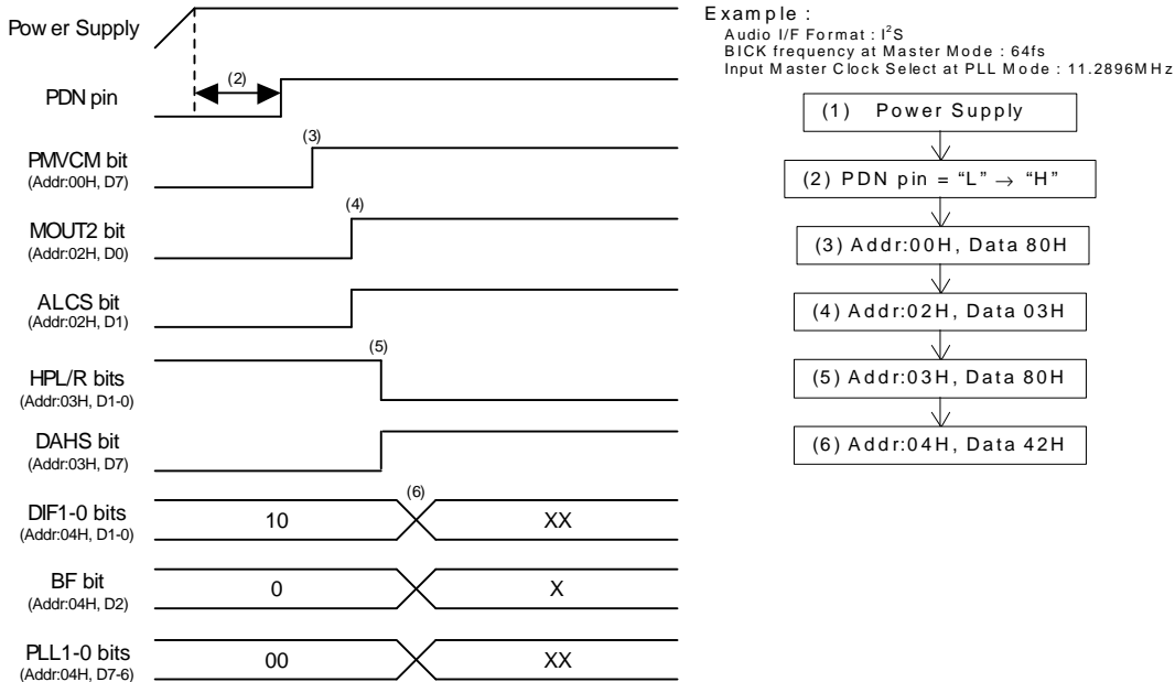
Figure 45. Power Up Sequence
