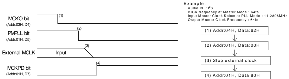
Figure 54. Stop of Clock Sequence(2)
