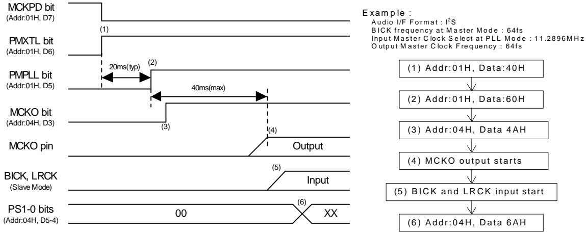
Figure 46. Clock Set Up Sequence(1)
