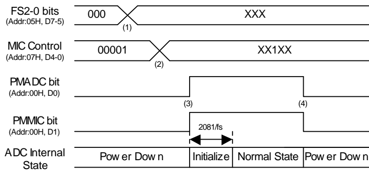
Figure 37. MIC Input Recording Sequence
