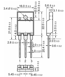
TO-3PML
