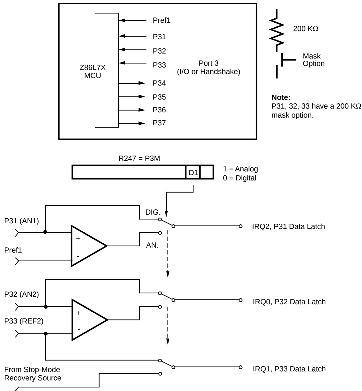
Figure 12. Port 3 Configuration
