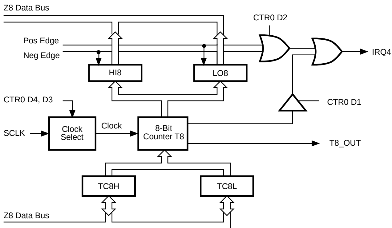
Figure 25. 16-Bit Counter/Timer Circuits
