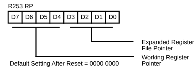
Figure 53. Register Pointer ((0) FDH: Read/Write)
