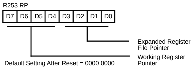
Figure 16. Register Pointer
