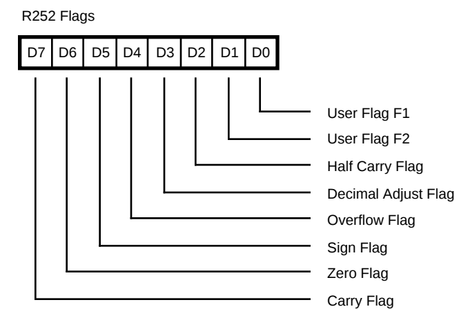
Figure 52. Flag Register ((0) FCH: Read/Write)
