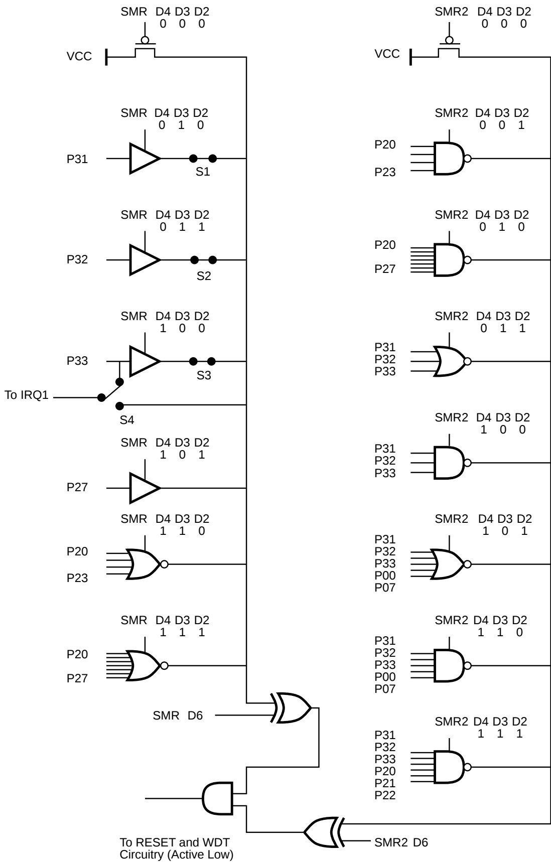
Figure 36. Stop-Mode Recovery Source
