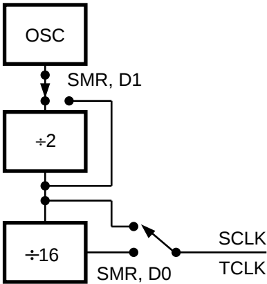
Figure 35. SCLK Circuit
