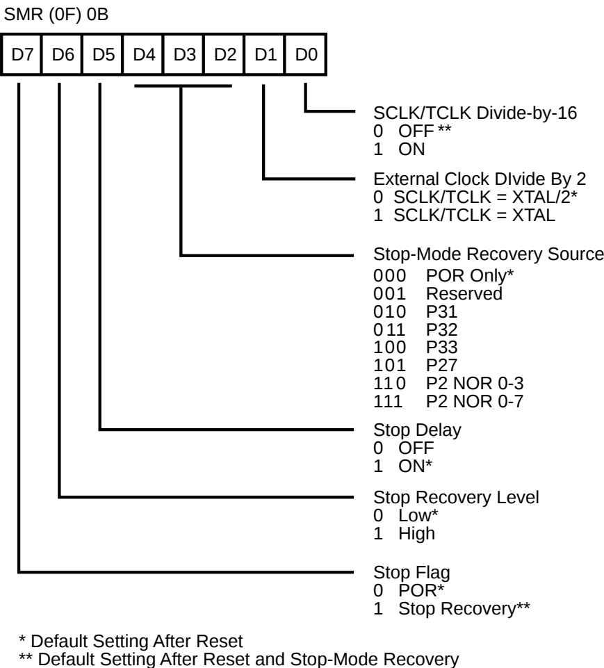
Figure 34. Stop-Mode Recovery Register
