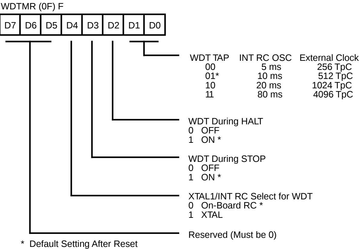
Figure 45. Watch-Dog Timer Mode Register (F) 0FH: Write Only
