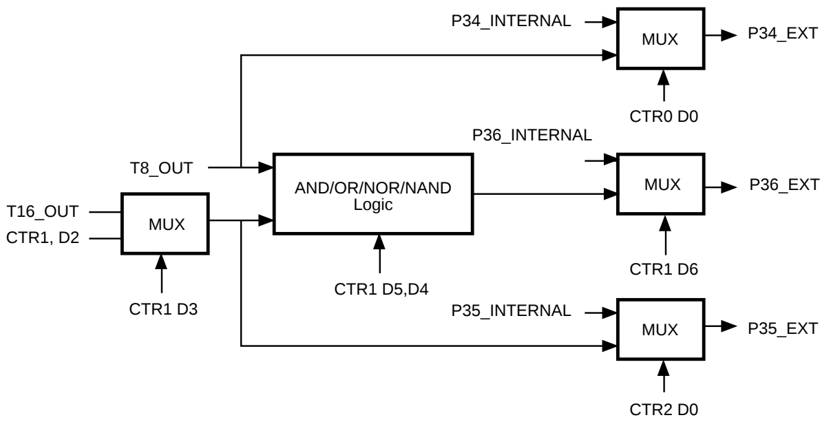
Figure 30. Output Circuit
