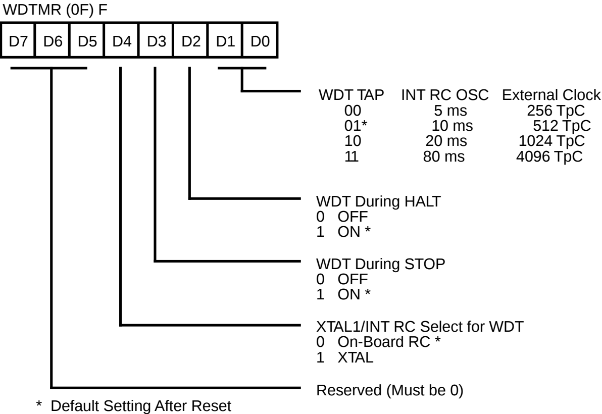
Figure 37. Watch-Dog Timer Mode Register (Write Only)
