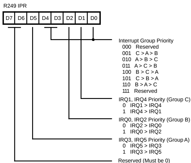
Figure 49. Interrupt Priority Registers ((0) F9H: Write Only)
