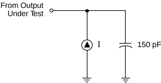
Figure 5. Test Load Diagram
