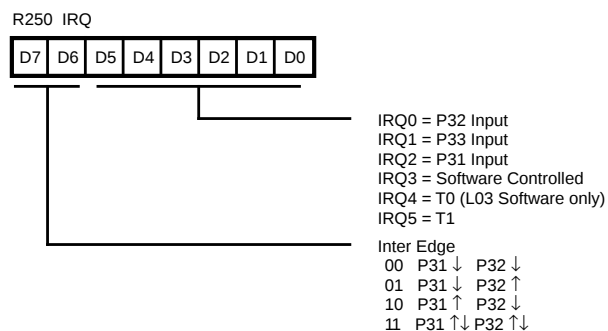
Figure 50. Interrupt Request Register ((0) FAH: Read/Write)
