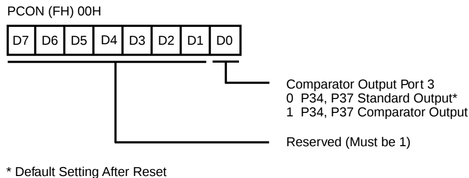
Figure 33. Port Configuration Register (PCON) (Write Only)
