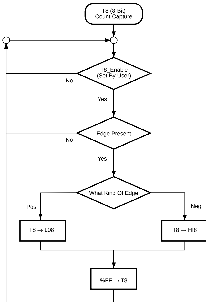
Figure 22. Demodulation Mode Count Capture Flowchart
