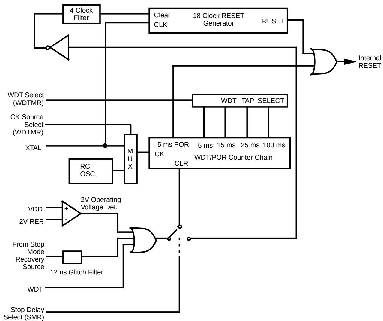
Figure 38. Resets and WDT
