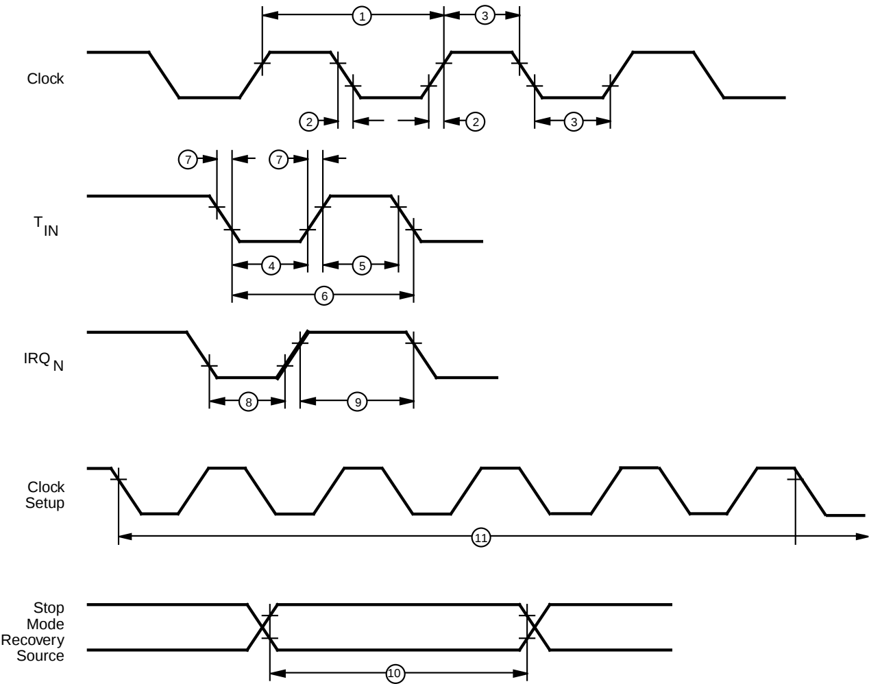
Figure 6. Additional Timing
