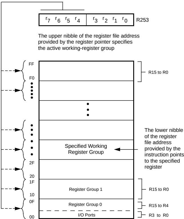
Figure 17. Register Pointer
