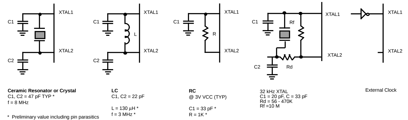
Figure 32. Oscillator Configuration
