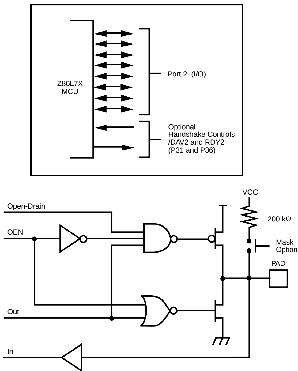
Figure 10. Port 2 Configuration
