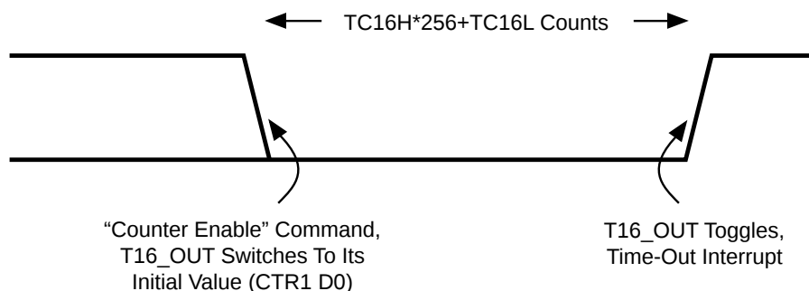
Figure 26. T16_OUT in Single-Pass Mode
