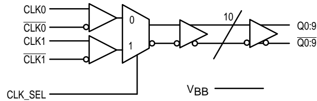
Figure 2. Logic Symbol
