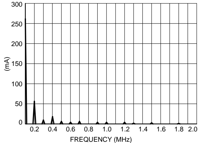
Figure 28. Continuous Conduction Mode
