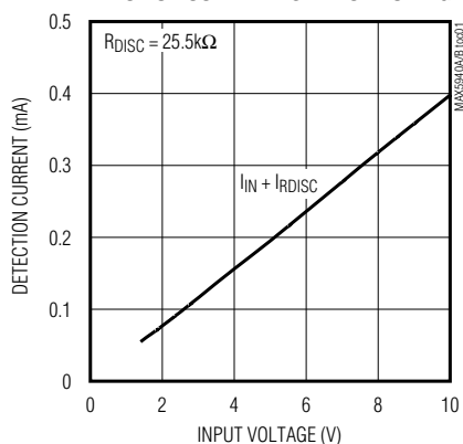
DETECTION CURRENT vs. INPUT VOLTAGE
