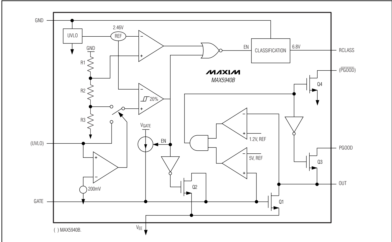
Figure 2. Block Diagram
