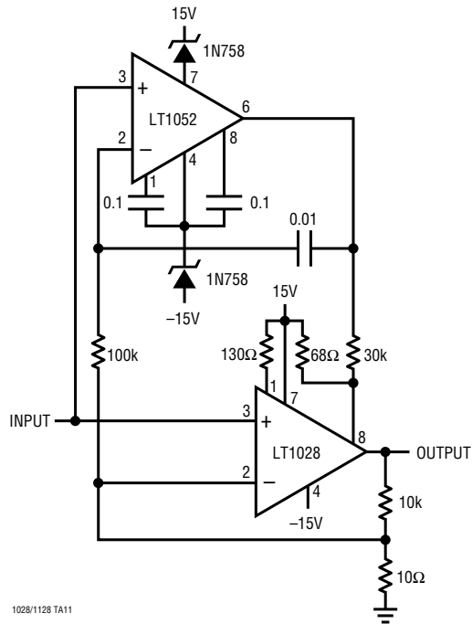
Chopper-Stabilized Amplifier
