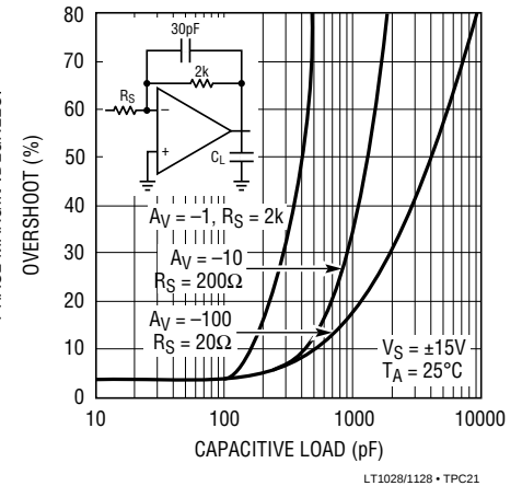
LT1028 Capacitance Load Handling
