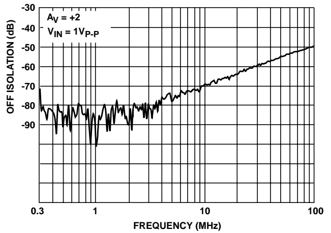
FIGURE 20. OFF ISOLATION
