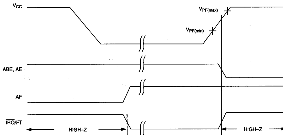
Figure 4. BACKUP MODE ALARM WAVEFORMS
