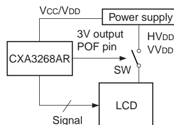
Fig. 2. System block diagram
