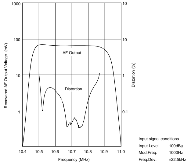
Frequency Characteristics
