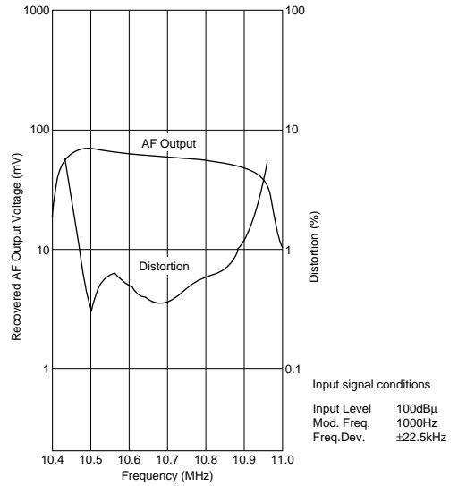
Frequency Characteristics
