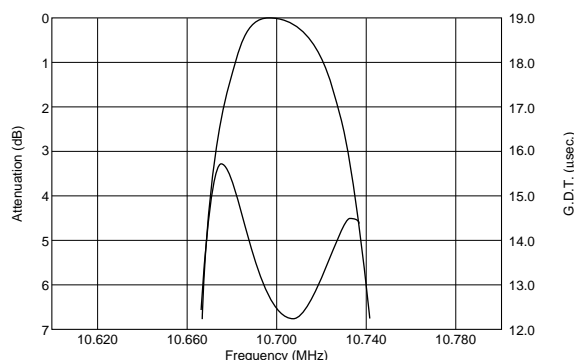
SFVLA10M7MF00-B0
