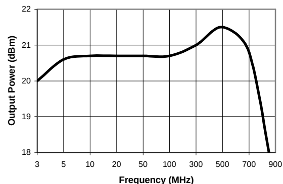
1 dB Compression
