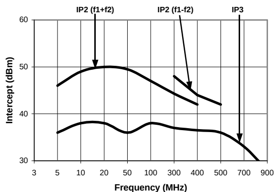
Intermodulation Intercept
