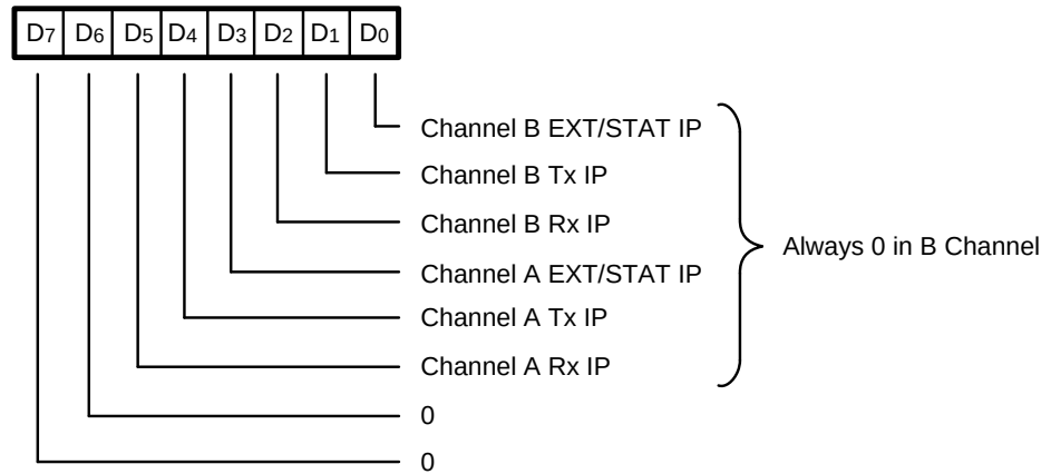
Figure 6–21. Read Register 3
