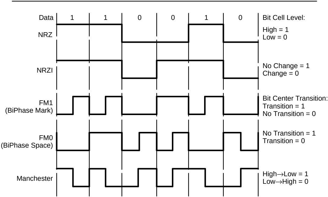
Figure 5–4. Data Encoding
