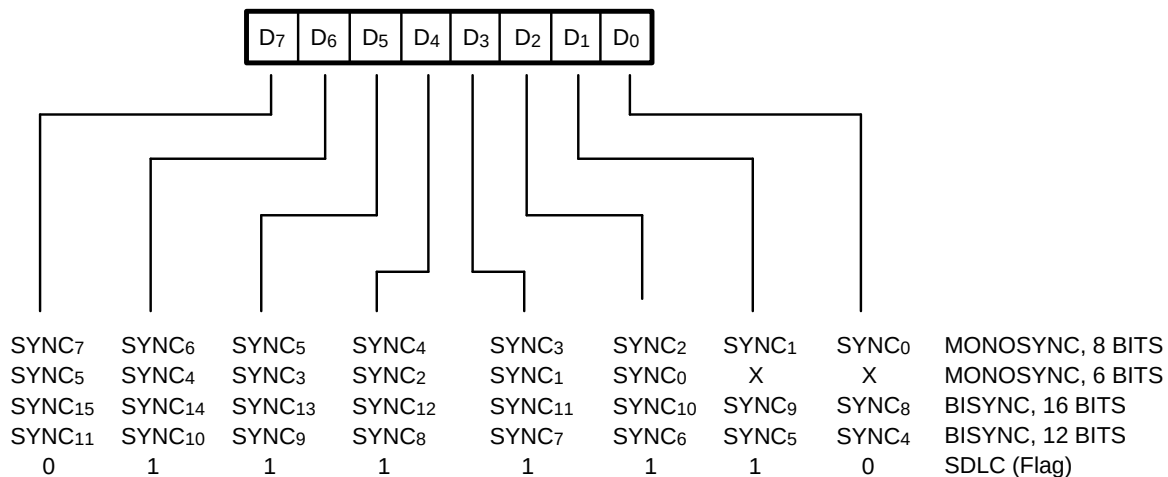
Figure 6-8. Write Register 7
