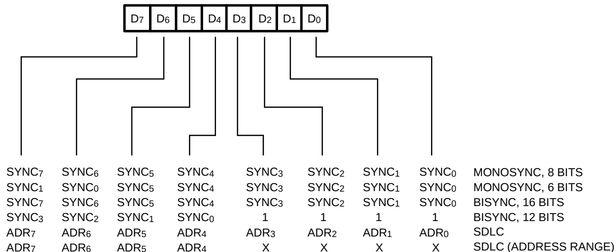
Figure 6-7. Write Register 6
