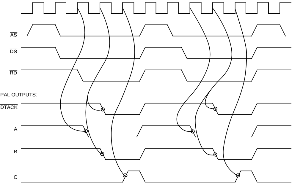
Figure 7–15. PAL Timing
