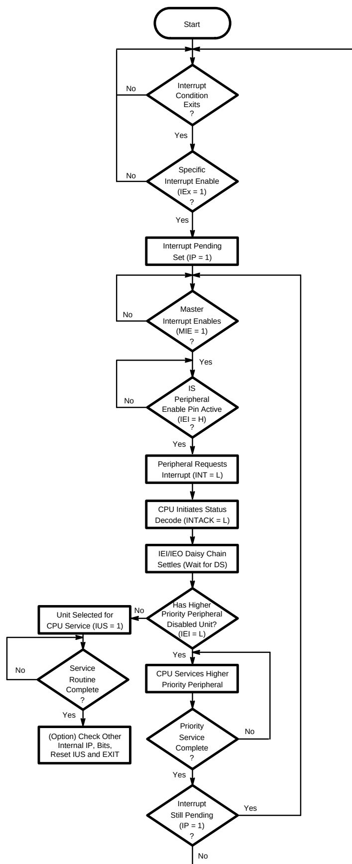
Figure 3-5. Interrupt Protocol
