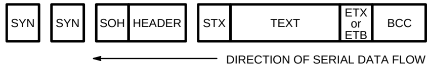
Figure 4–22. BISYNC Message Format
