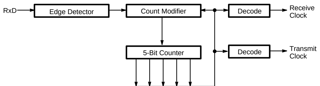
Figure 5–5. DPLL
