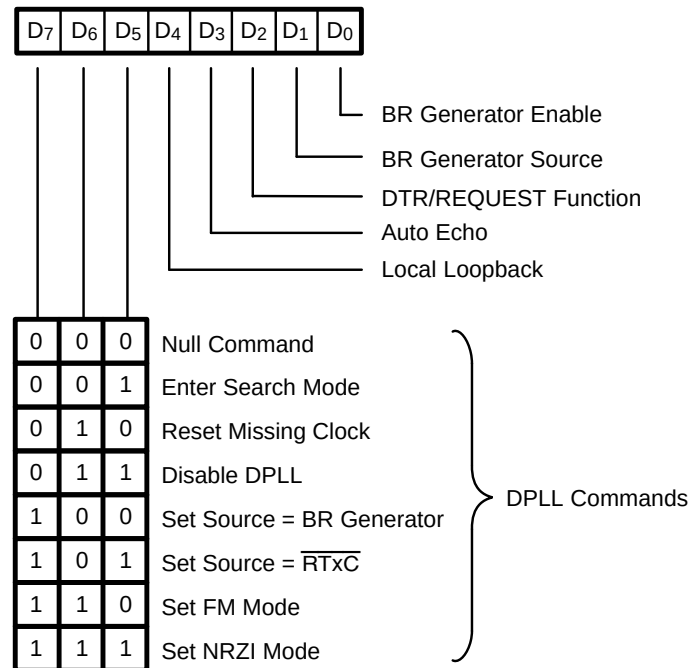
Figure 6–16. Write Register 14
