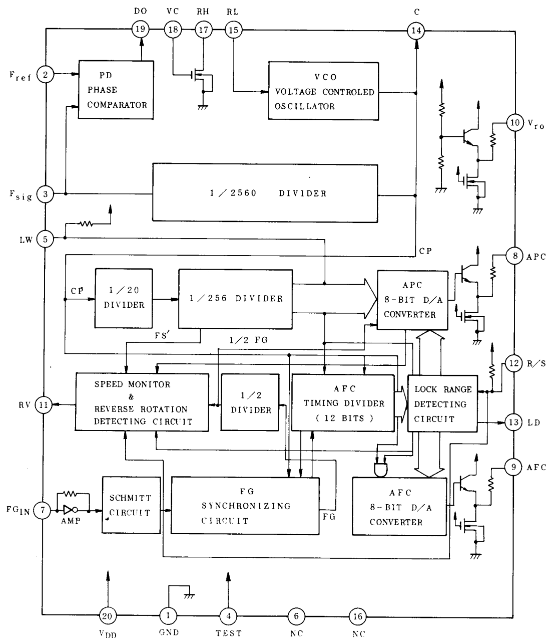
BLOCK DIAGRAM TC9192F
