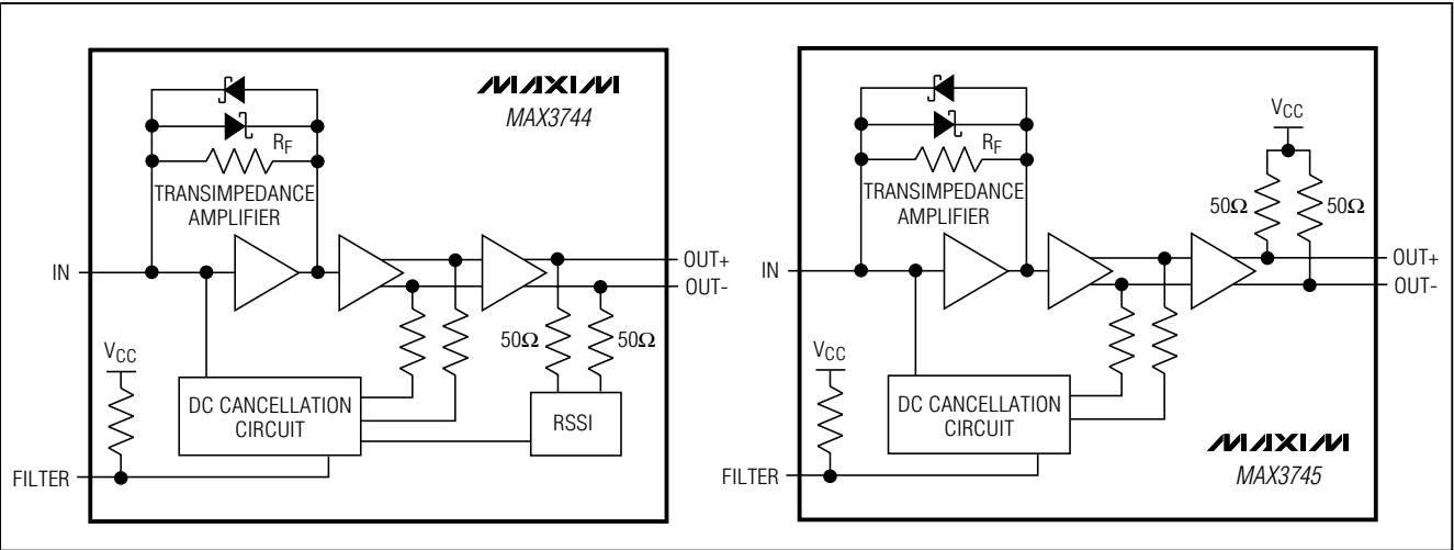
Figure 1. Functional Diagram
