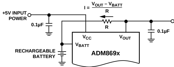
Figure 18. Rechargeable Battery
