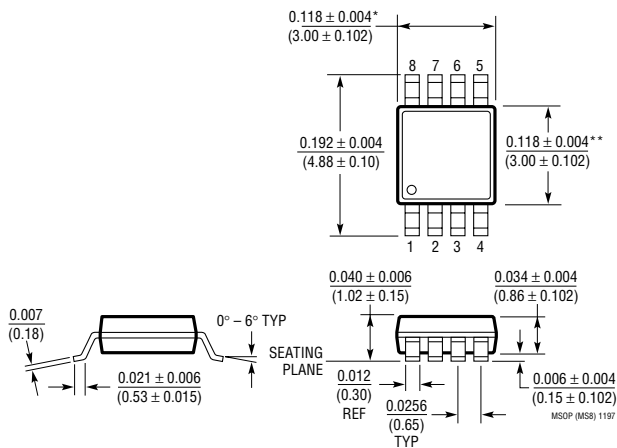
MS8 Package 8-Lead Plastic MSOP (LTC DWG # 05-08-1660)
