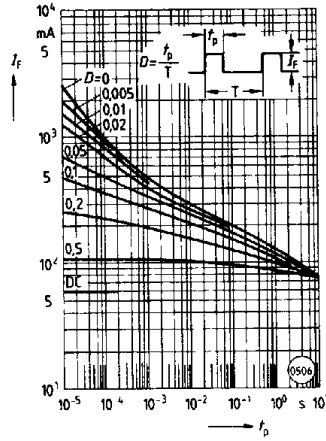
Permissible pulse handling capability Forward current versus pulse width ( D =parameter, T_A=25^\circ\text{C} )
