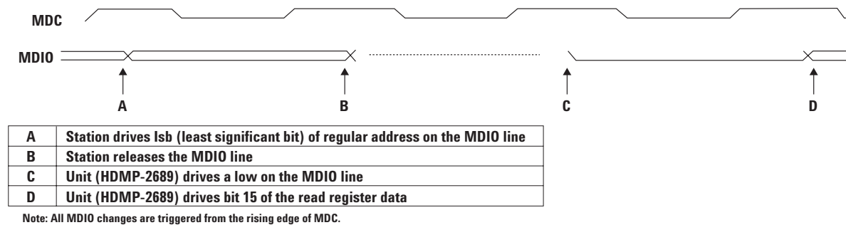
MDIO Timing, Turn Around (TA) Cycles During a Read.
