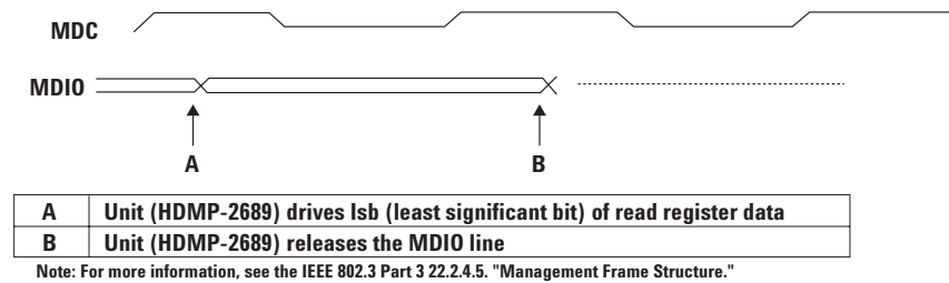
MDIO Timing, Last Bit of Read Register Data, Bus Released by the HDMP-2689.
