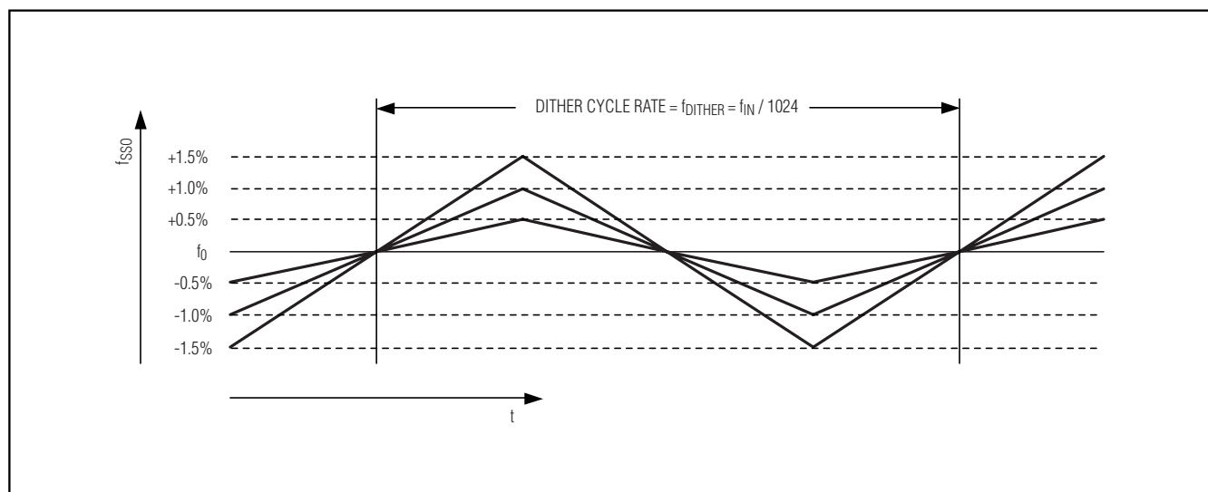
Figure 1. Spread-Spectrum Frequency Modulation
