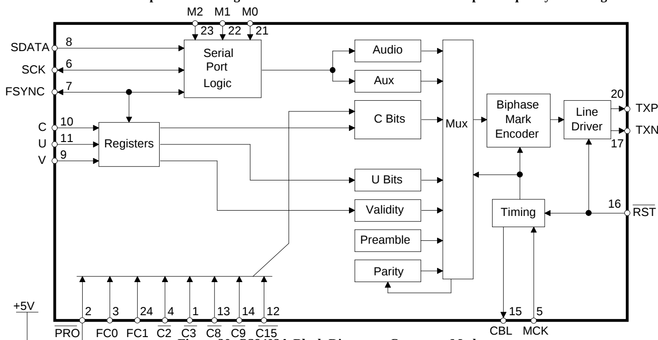
Figure 20. CS8402A Block Diagram - Consumer Mode
