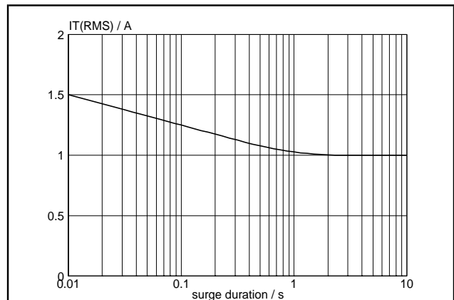
Fig.5. Maximum permissible repetitive rms on-state current I_{T(RMS)} , versus surge duration, for sinusoidal currents, f = 50\text{ Hz} ; T_{sp} \leq 108^\circ\text{C} .
