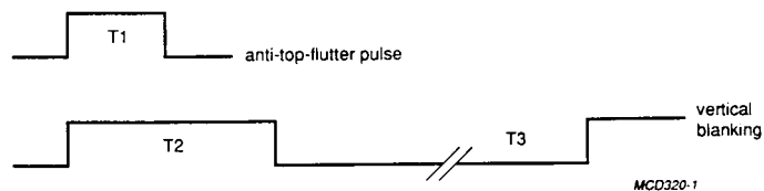
Fig.8 Anti-top-flutter-pulse.
