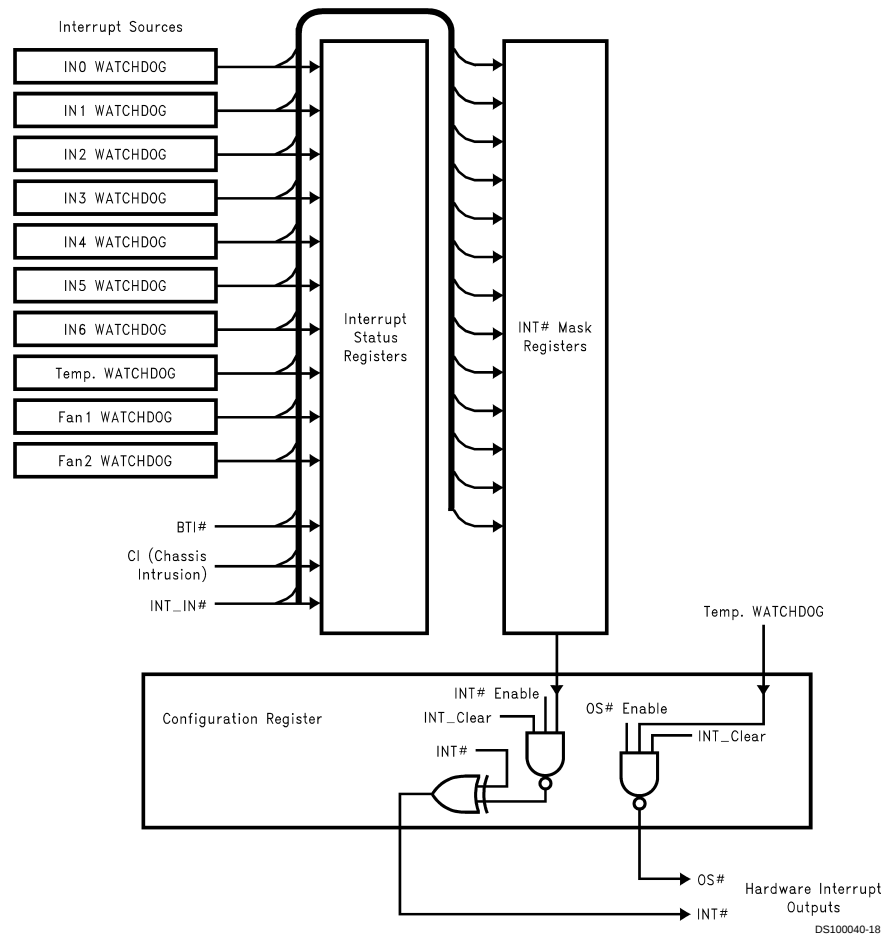
FIGURE 10. Interrupt Structure
