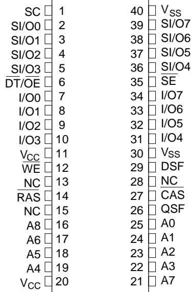
HM538123BJ Series
