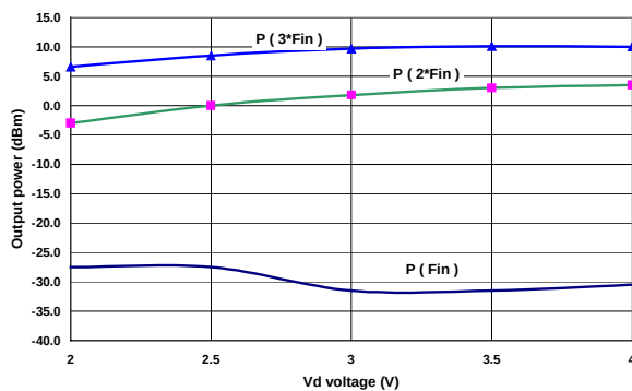
Pout versus Vd @ Pin=14dBm &amp; Fin=13GHz
