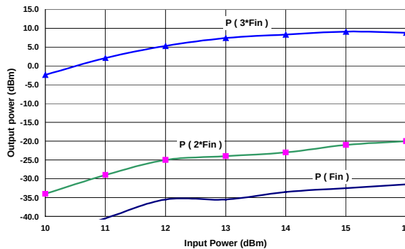
Pout versus Pin @ Fin=12GHz &amp; Vd=3V
