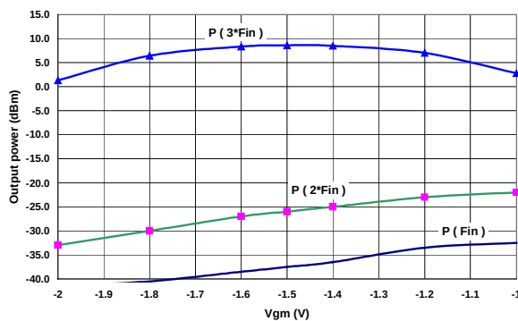
Pout versus Vgm @ Fin=12GHz &amp; Vd=3V
