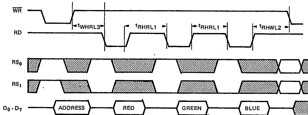
Figure 13. Color Value Read Followed by any Write.
