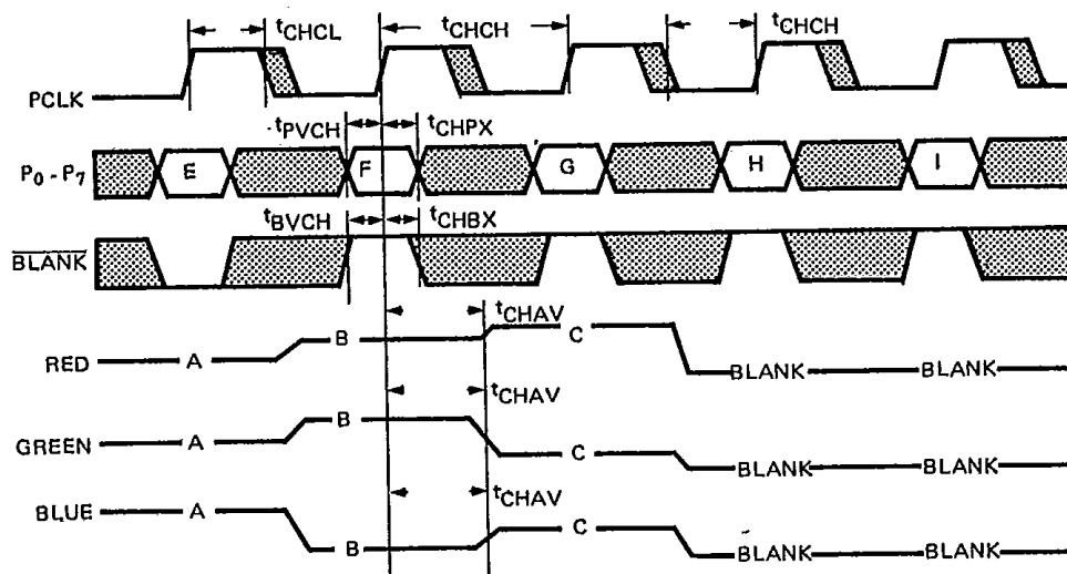
Figure 2. Timing Diagram Detailing Timing Specifications.
