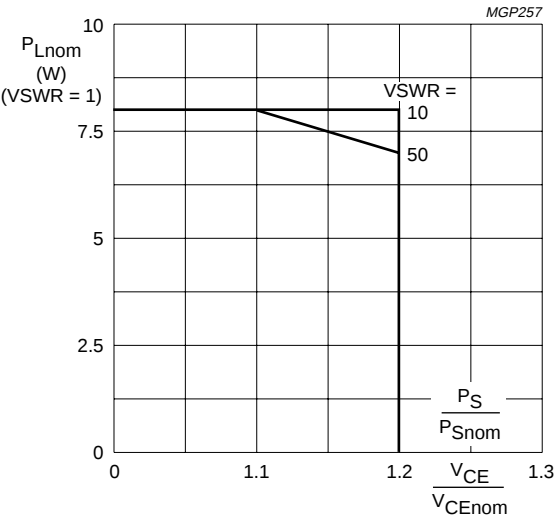
Fig.11 R.F. SOAR (short-time operation during mismatch); f = 175 MHz; T_h = 70 °C; R_{th\,mb-h} = 0.3 K/W; V_{CEnom} = 13.5 V or 12.5 V; P_S = P_{Snom} at V_{CEnom} and VSWR = 1 .
