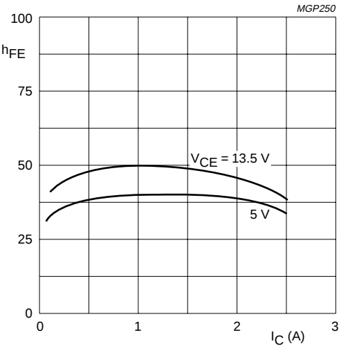
Fig.4 Typical values; T_j = 25\text{ }^{\circ}\text{C} .
