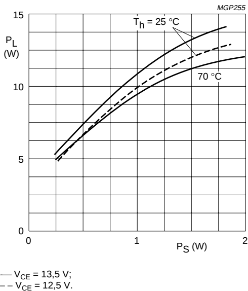
Fig.9 Typical values; f = 175 MHz;
