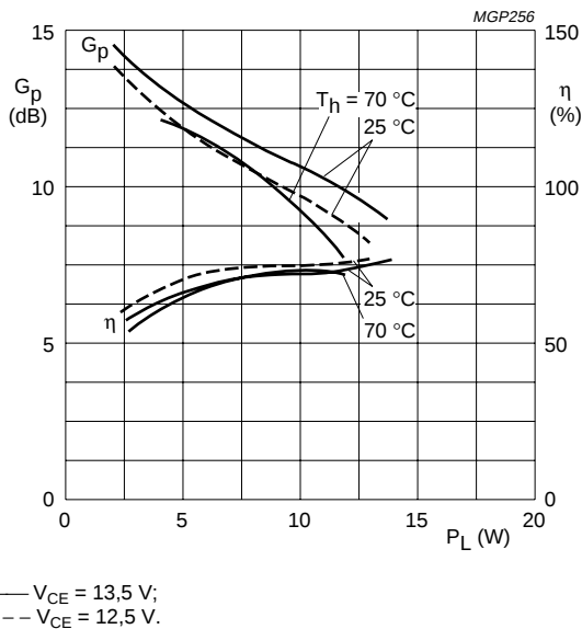
Fig.10 Typical values; f = 175 MHz;
