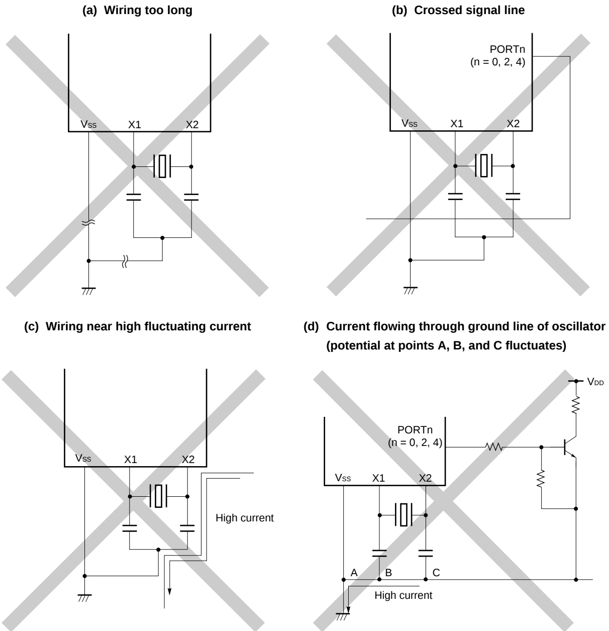
Figure 7-4. Examples of Incorrect Resonator Connection (1/2)
