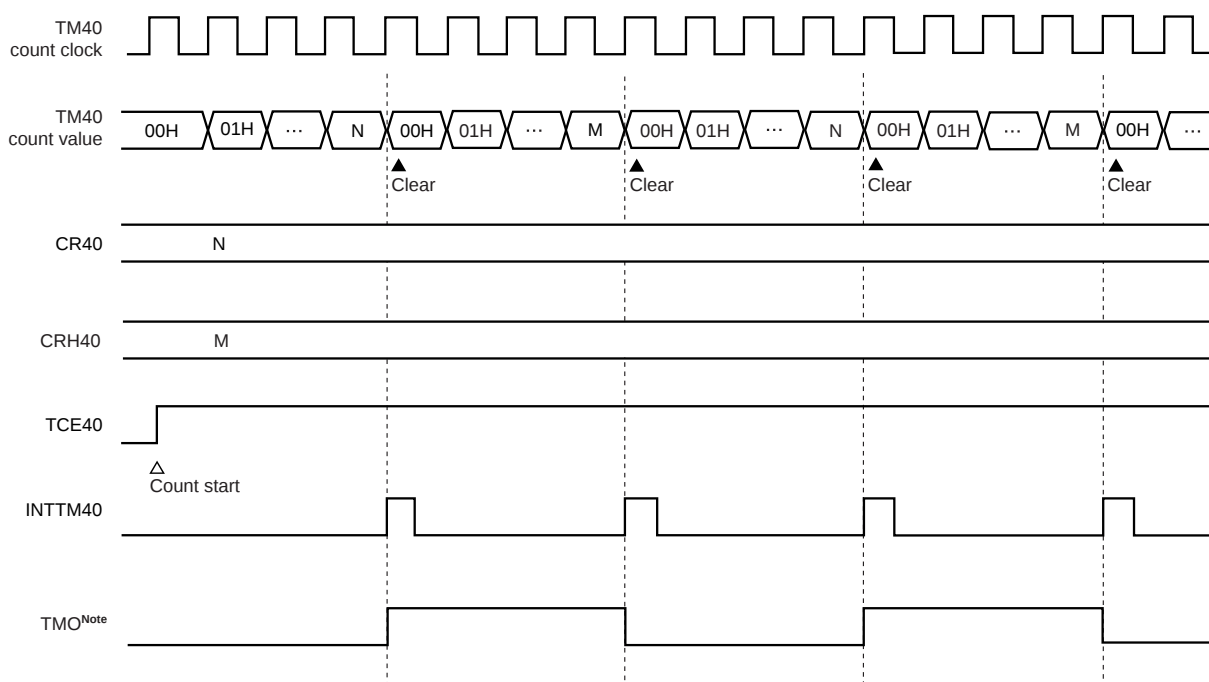
Figure 9-22. PWM Output Mode Timing (Basic Operation)
