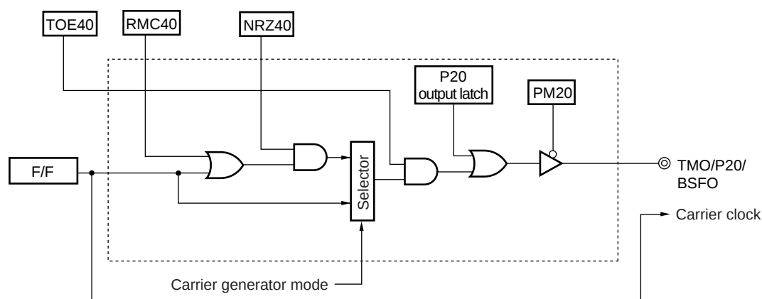
Figure 9-3. Block Diagram of Output Controller (Timer 40)
