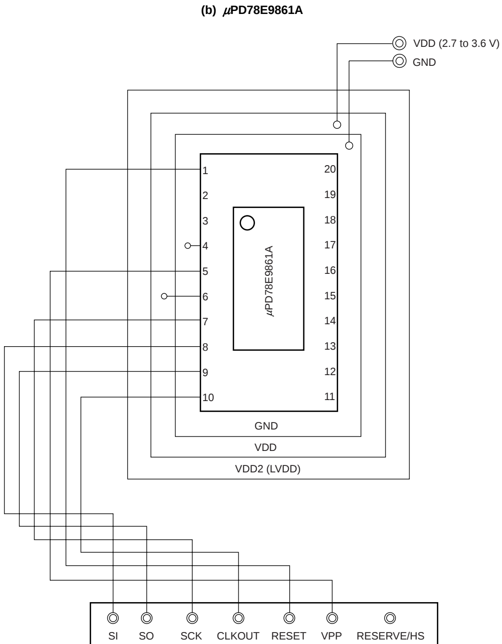
Figure 17-8. Wiring Example for EEPROM Writing Adapter with Pseudo 3-Wire (2/2)
