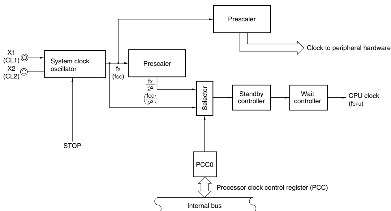
Figure 6-2. Clock Generator Block Diagram
