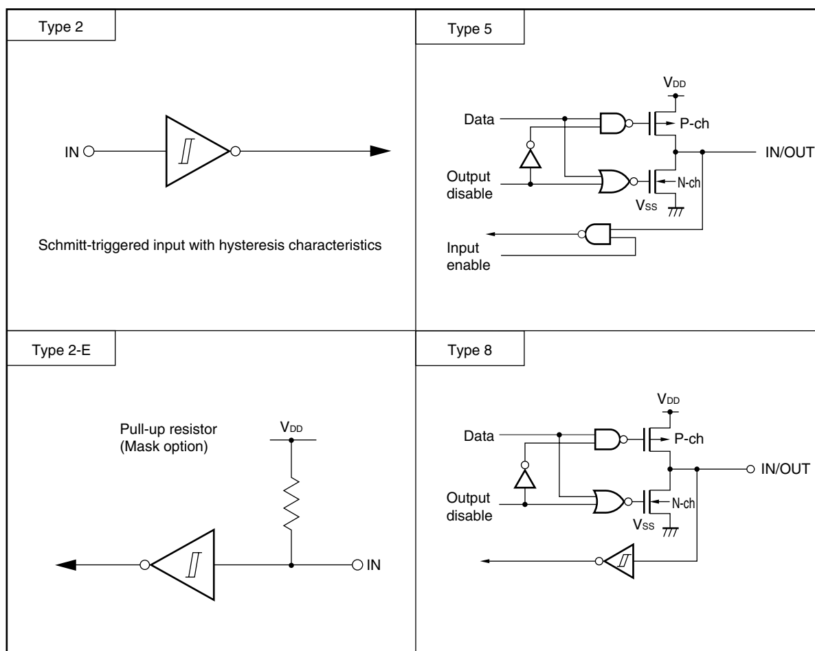
Figure 3-1. Pin I/O Circuits
