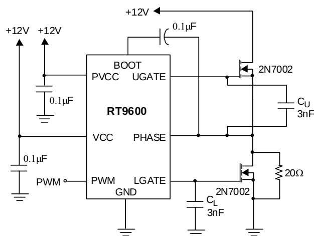
Testing Circuit
