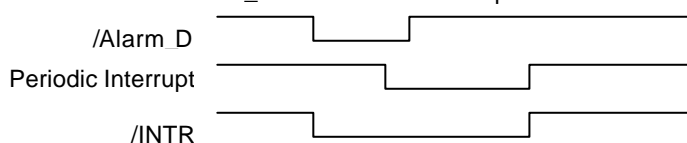
Example: Combined Output to /INTR Pin Under Control of /ALARM_D and Periodic Interrupt
