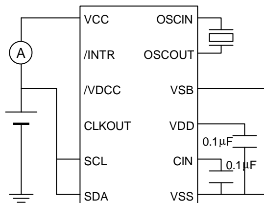
Test circuit
