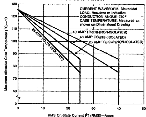
FIGURE 1B — Maximum Allowable Case Temperature vs On-State Current
