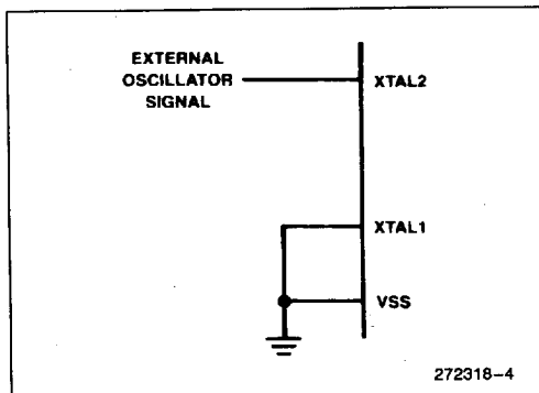
Figure 4. External Drive Configuration
