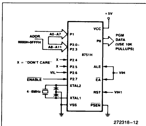
Figure 6. Program Verification
