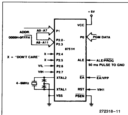
Figure 5. Programming Configuration
