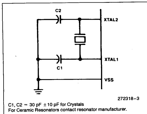
Figure 3. Oscillator Connections
