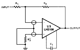
INVERTING AMPLIFIER
