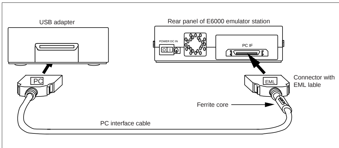
Figure 4 Connecting USB adapter to E6000 Emulator
