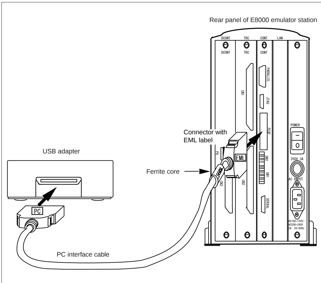
Figure 5 Connecting USB Adapter to E8000 Emulator
