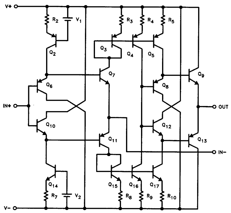
Equivalent Circuit (One of Two Amplifiers)
