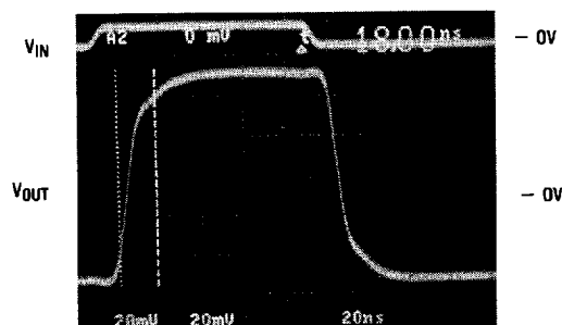
Small Signal Response
