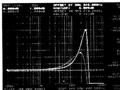
EL2232 Frequency response with and without 150Ω/100 pF output snubber C_L = 68 \text{ pF}
