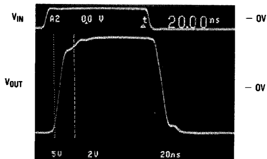
Large Signal Response
