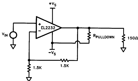
Adding a Pulldown Resistor to Improve Video Performance
