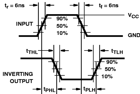
FIGURE 6. HC AND HCU TRANSITION TIMES AND PROPAGATION DELAY TIMES, COMBINATION LOGIC
