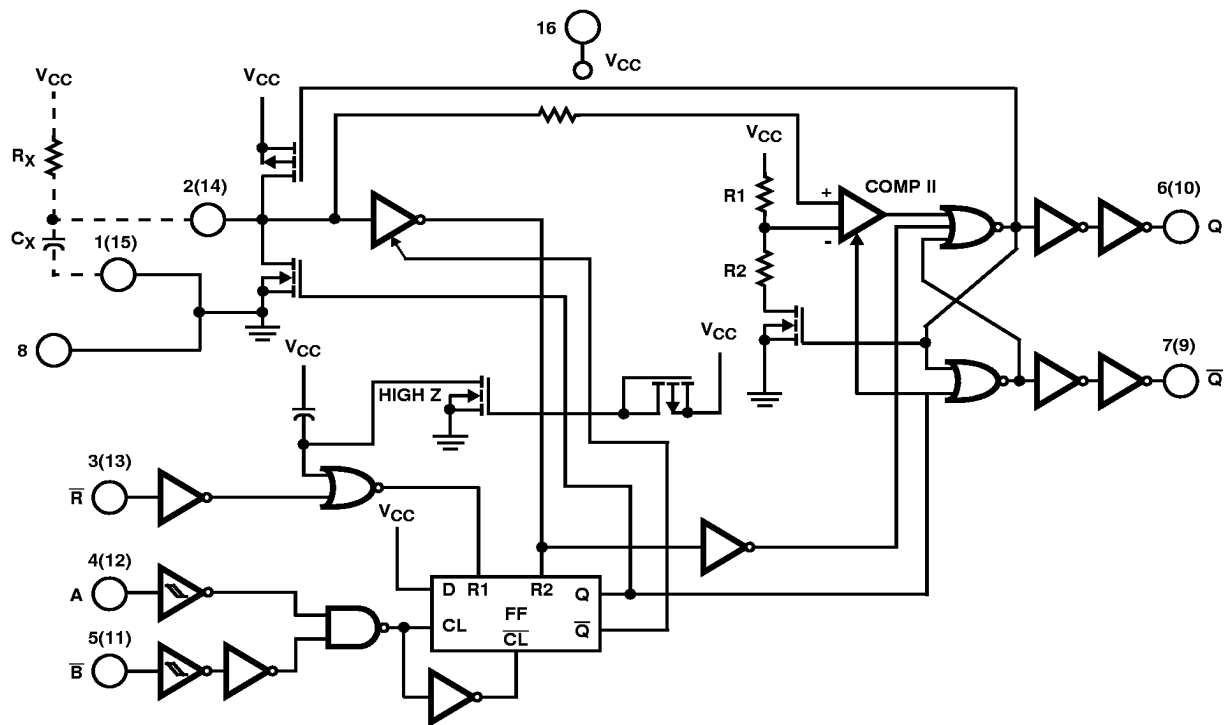
FIGURE 2. LOGIC DIAGRAM (1 MONO)
