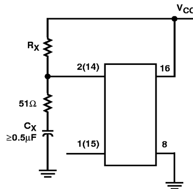
FIGURE 13. ALTERNATE RAPID POWER-DOWN PROTECTION CIRCUIT
