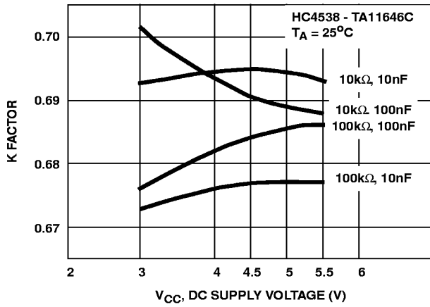
FIGURE 8. K FACTOR vs DC SUPPLY VOLTAGE (V CC ) - V
