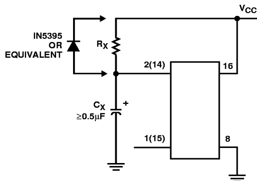
FIGURE 12. RAPID POWER-DOWN PROTECTION CIRCUIT
