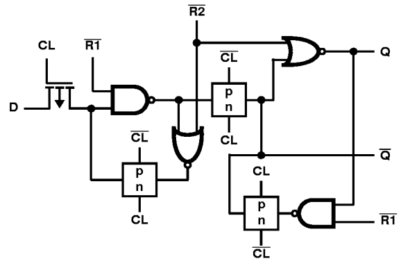
FIGURE 1. FF DETAIL
