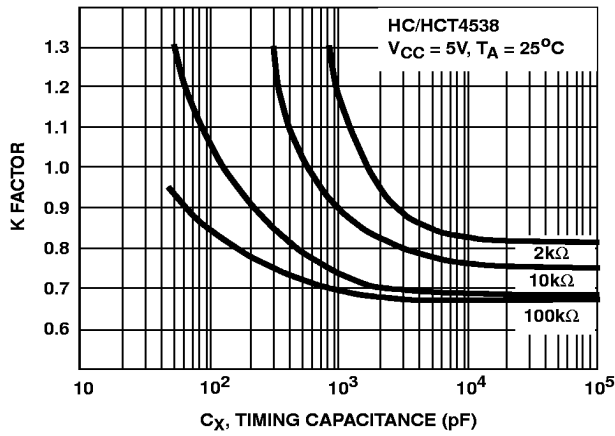
FIGURE 10. K FACTOR vs C X
