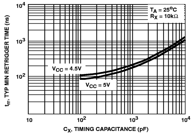
FIGURE 11. MINIMUM RETRIGGER TIME vs TIMING CAPACITANCE
