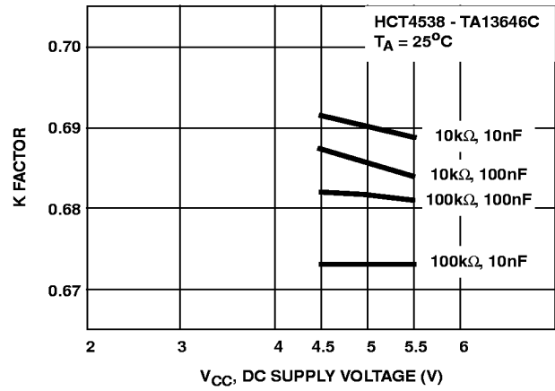
FIGURE 9. K FACTOR vs DC SUPPLY VOLTAGE (V CC ) - V
