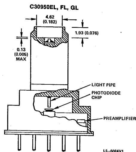
Figure 3 - Cutaway of Package
