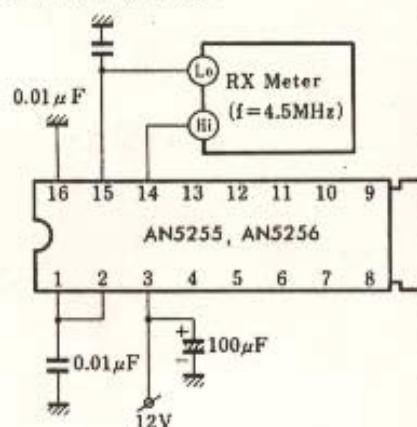
Test Circuit 2 ( R_i, C_i )
