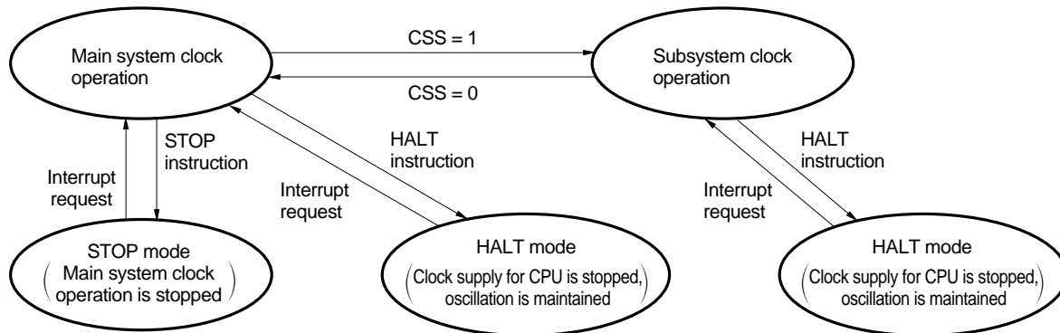
Figure 8-1. Standby Function
