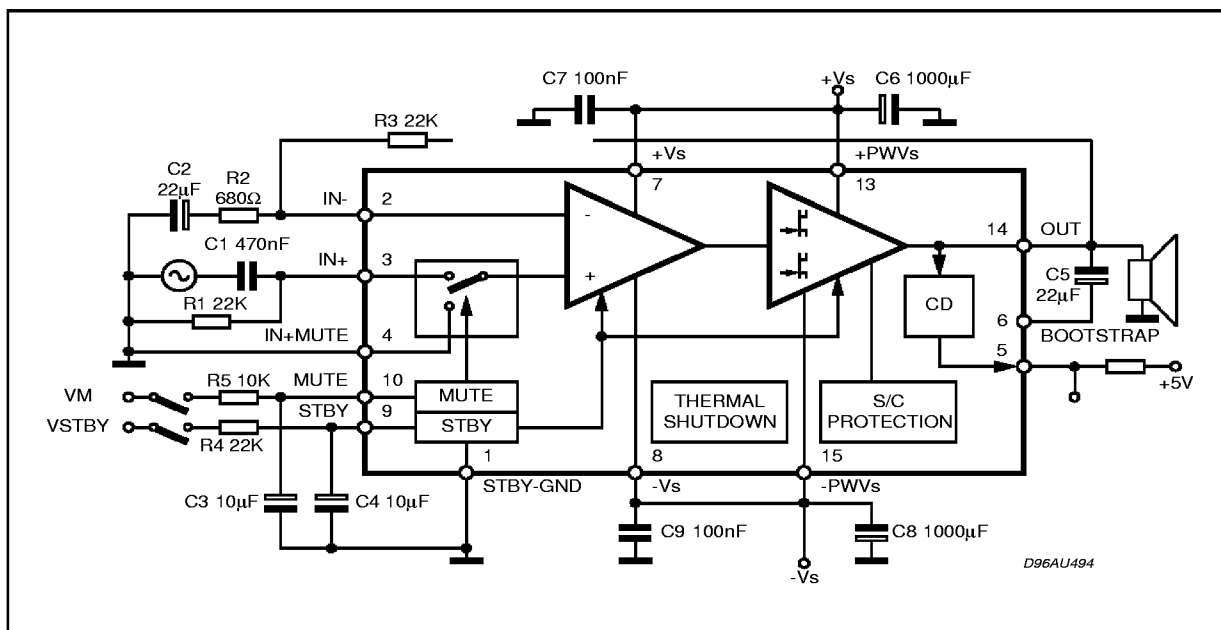
Figure 1: Typical Application and Test Circuit
