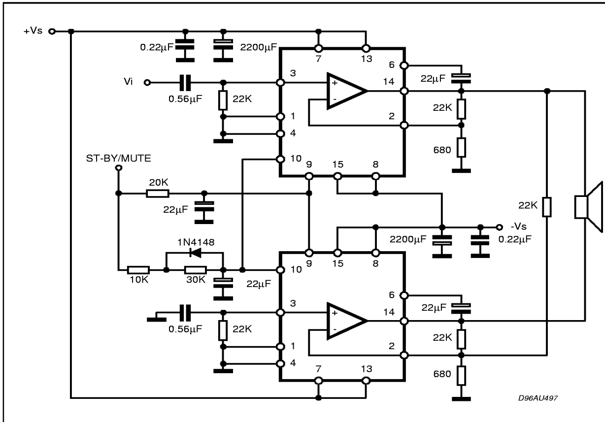
Figure 19: Bridge Application Circuit
