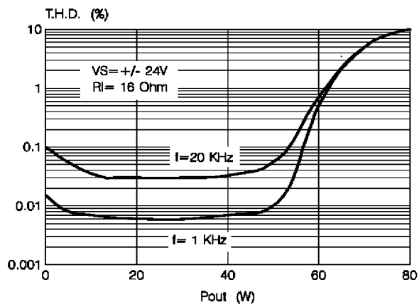
Figure 22: Distortion vs. Output Power
